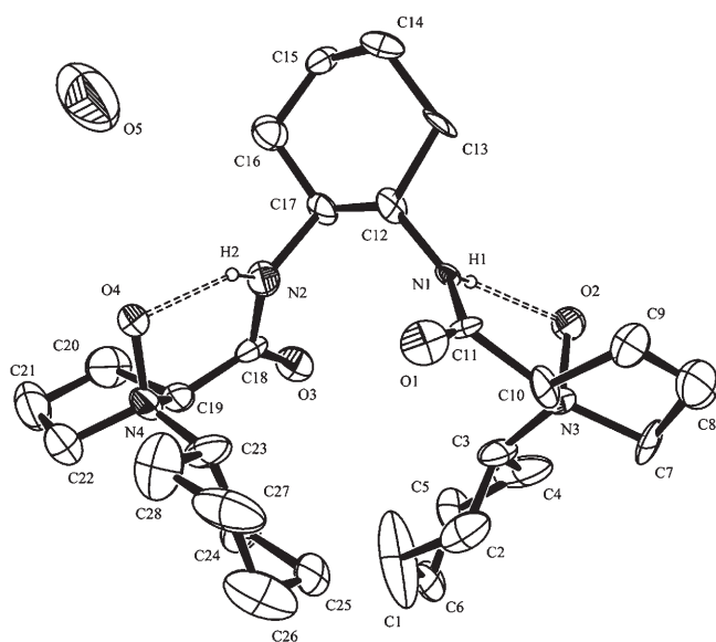
Figure 2. X-ray crystal structure of N,N' -dioxide 1c ·H 2 O.
