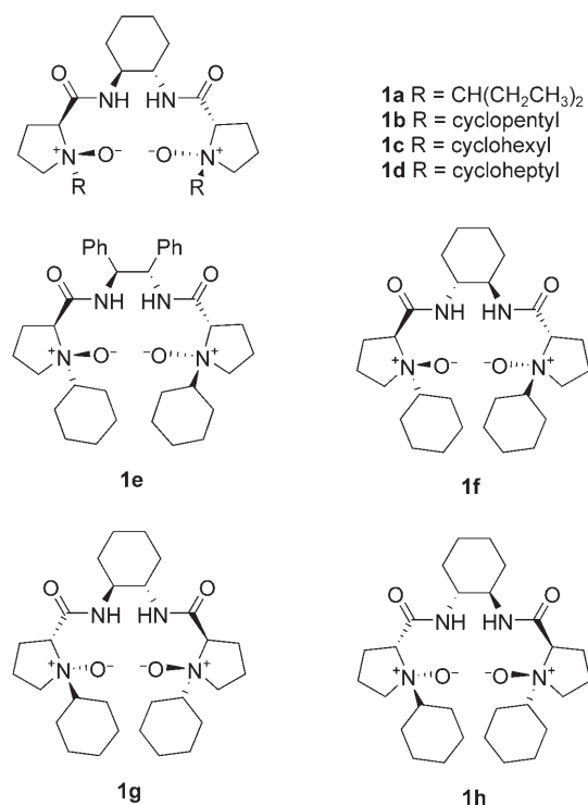
Figure 1. N,N' -dioxides 1a–h .
