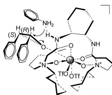
Figure 3. Proposed transition state model.
